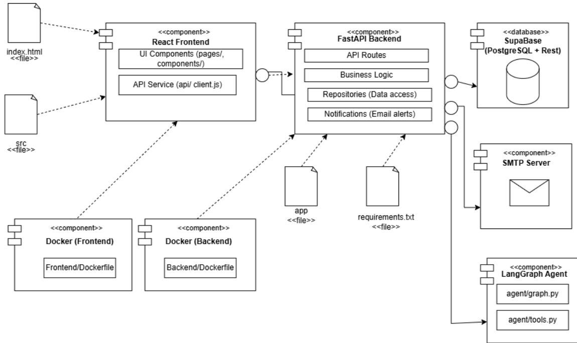
Figure 2.13: Component Diagram of the AI-Powered Student Workload Balancer
